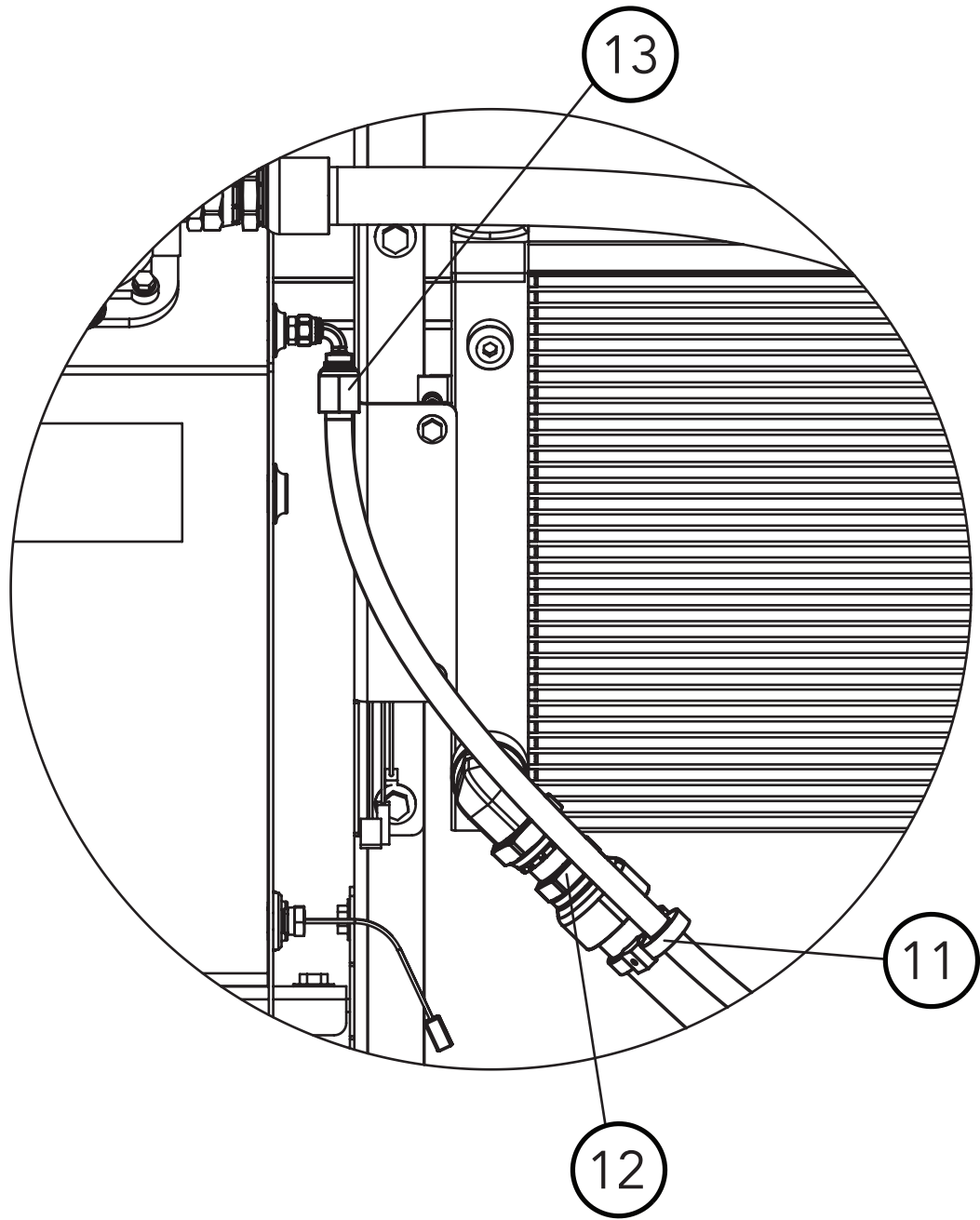
Detail D
