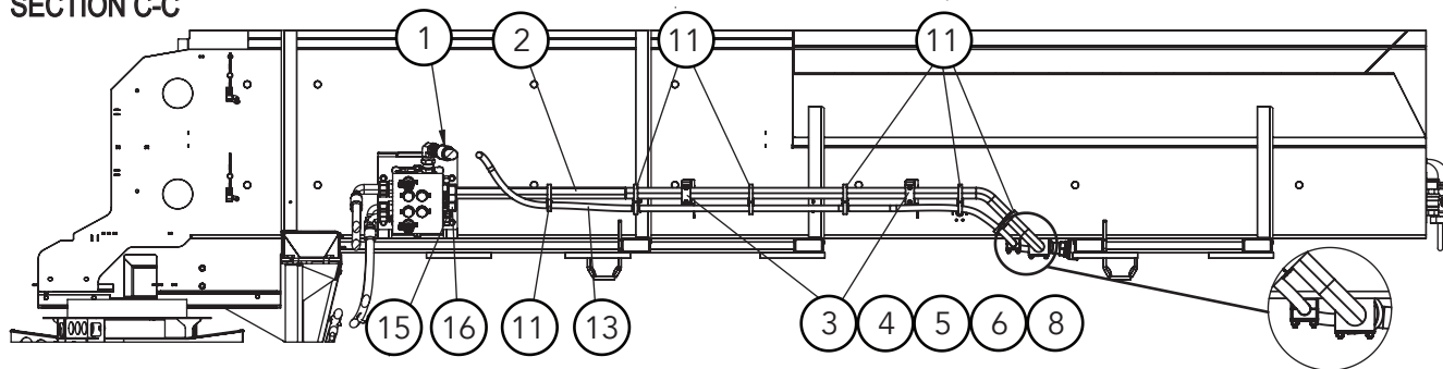
SECTION C-C
