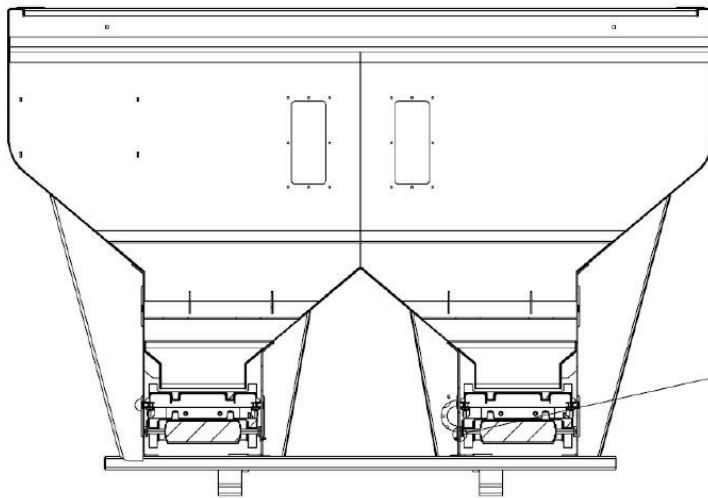
SECTION G-G
