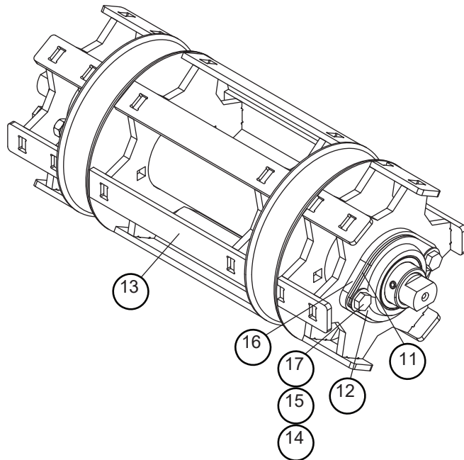
Tail Pulley
