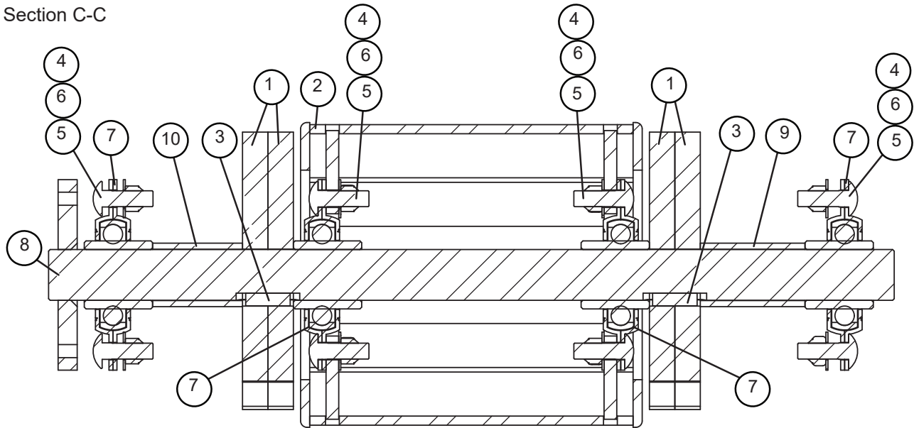
Tail Pulley
